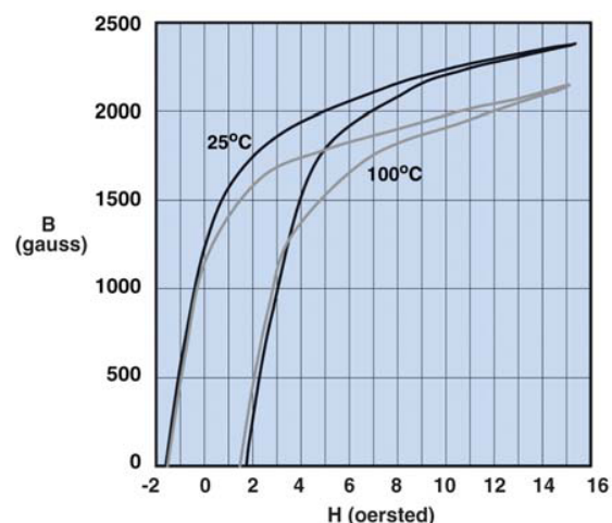
Hysteresis Loop
